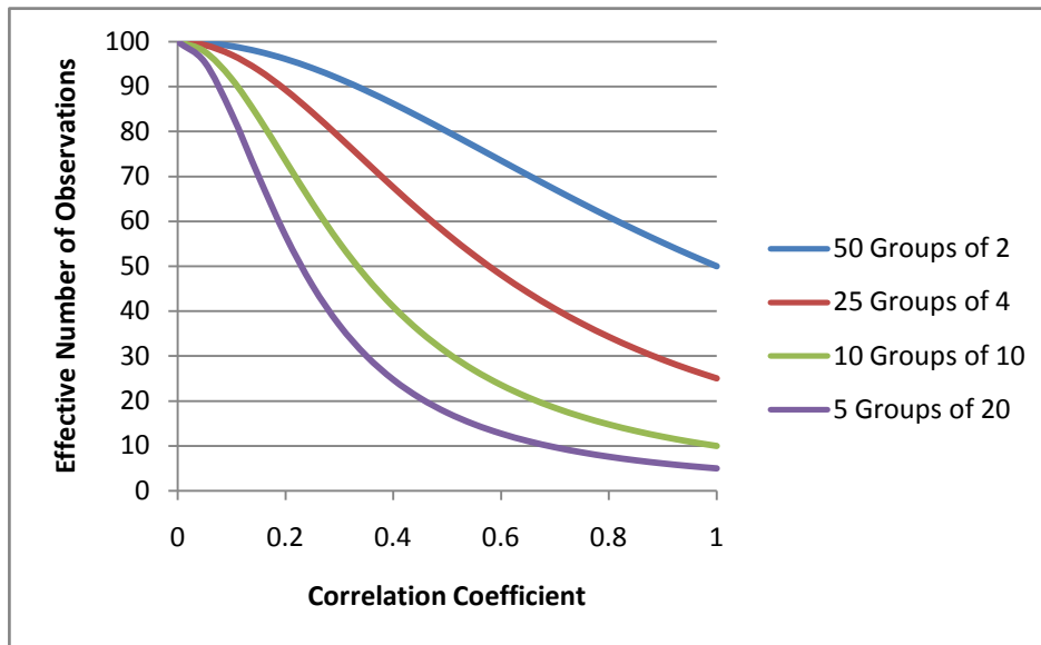
Figure 6.3. Correlation and Effective Number of Observations
